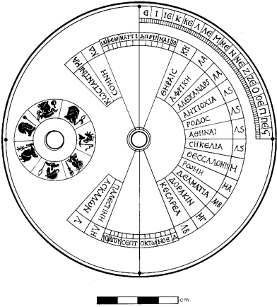
Geared sundial-calendar Greco-Roman, 5th-6th c London, Science Museum
