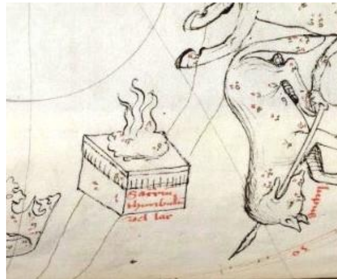
southern hemisphere
