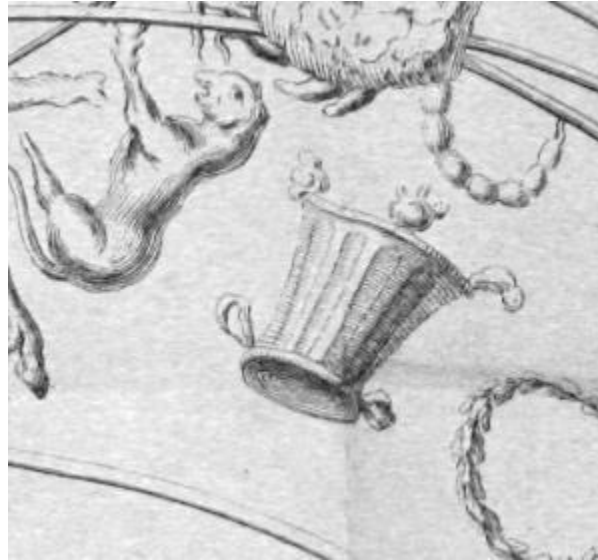
Bentley's Manilius
