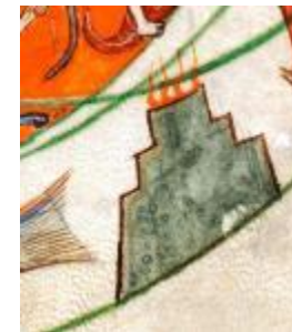
vs. planisphere
