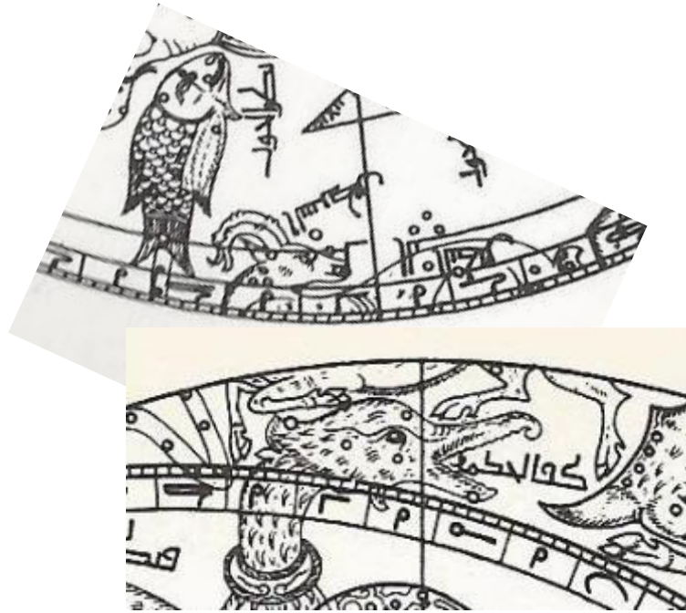
BM, Malcolm globe
