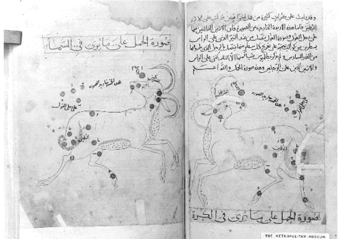
NY, Metropolitan Mus Ms Rogers Fund 1913 c. 1400, Samarkand
