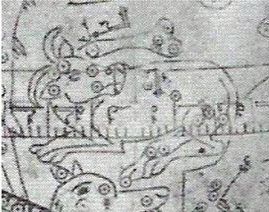
Florence, Mus delle Scienze, no. 2712 - dated 1025 AD n.b. – seated to left, head back
