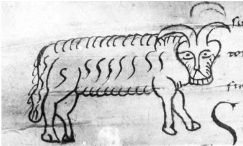
Paris BN n.a. 1614 – walking to right, facing viewer, lyre horns
