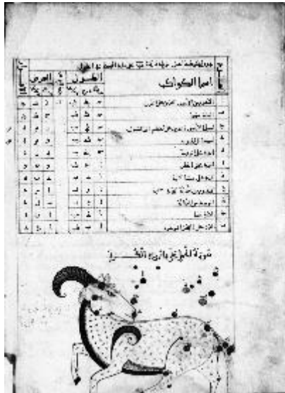
Vatican, BAV Ross 1033 1224 AD, Ceuta (?) N Africa similar
