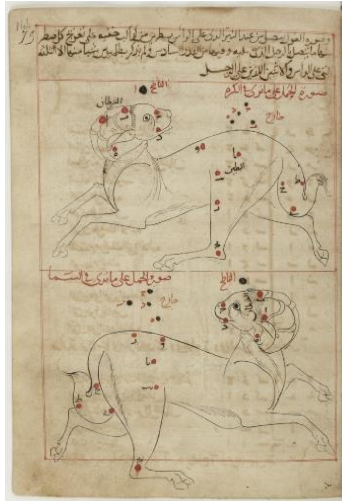
Paris BN Arabe 2489 1266-67 AD; Syria? n.b. – leaping, head back
