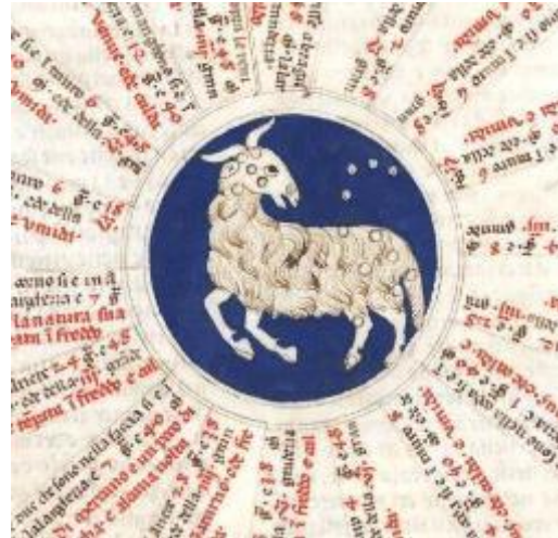
Vatican BAV Vat lat 8174 n.b. – trots to left, head back ... E chiamasi in latinio aries e in arabico alhamal
