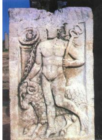
Hermes with Ram 3rd C BC Ephesus, Pyrtaneion
