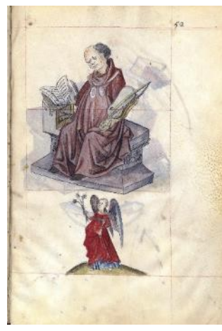
Mercury – exaltation
