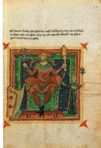
Mercury – exaltation
