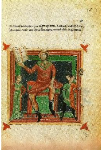
Mercury – domus
